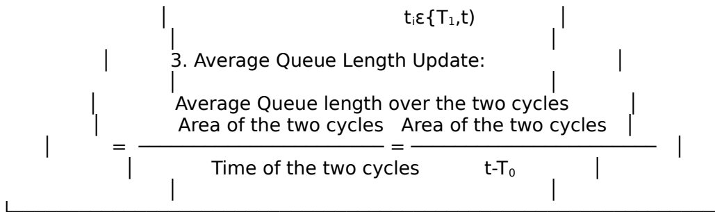
Figure 1 - Queue length averaging algorithm
