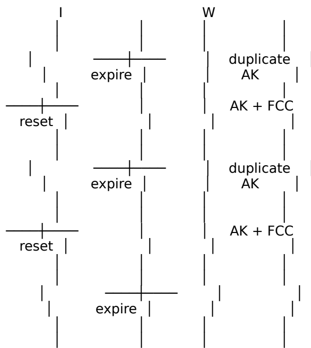
Figure 1 - AK exchange on idle connection.
