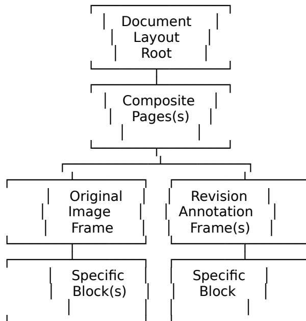
Figure 2 - Document layout structure
