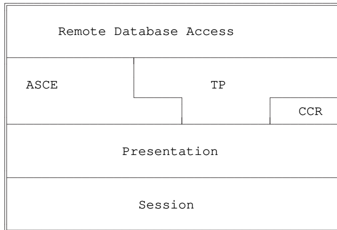
Figure 1 - Placement of RDA within the application layer
