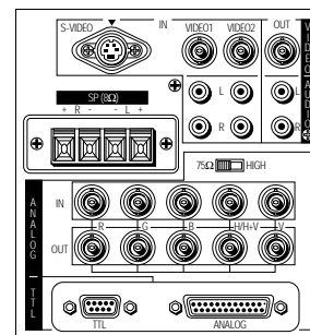
MegaView 29 Connector Panel
