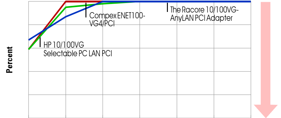
CPU UTILIZATION
