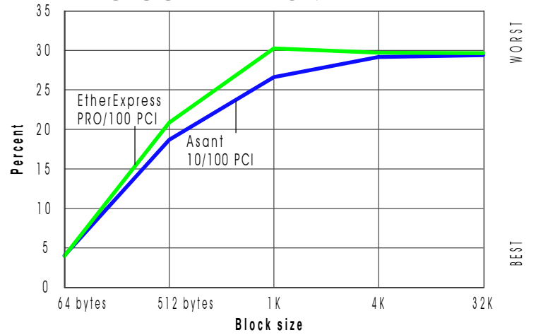
CPU UTILIZATION
