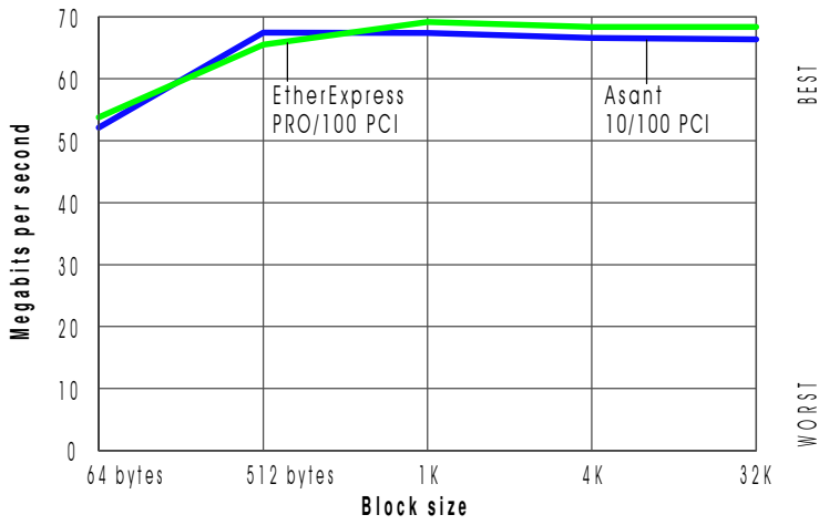
NIC THROUGHPUT
