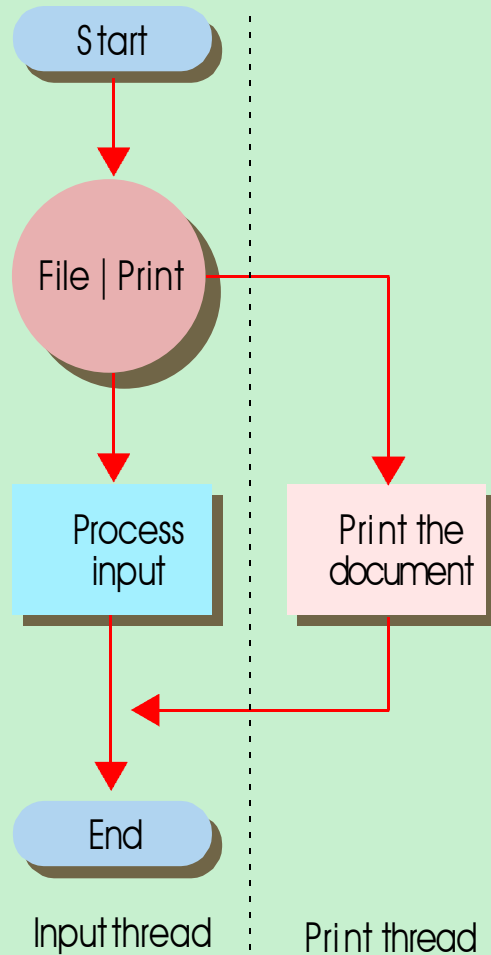
Multiple threads
