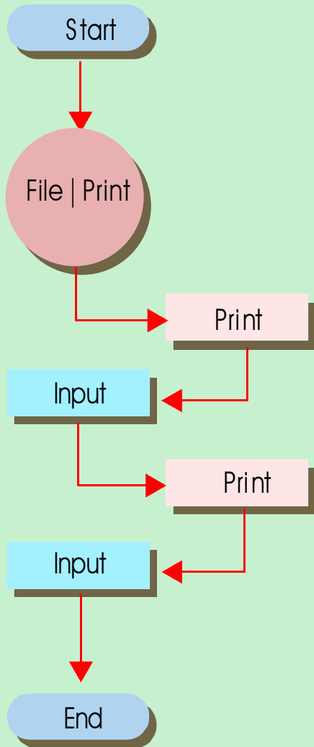
Single thread
