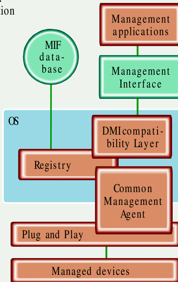
Windows 95 partial DMI implementation
