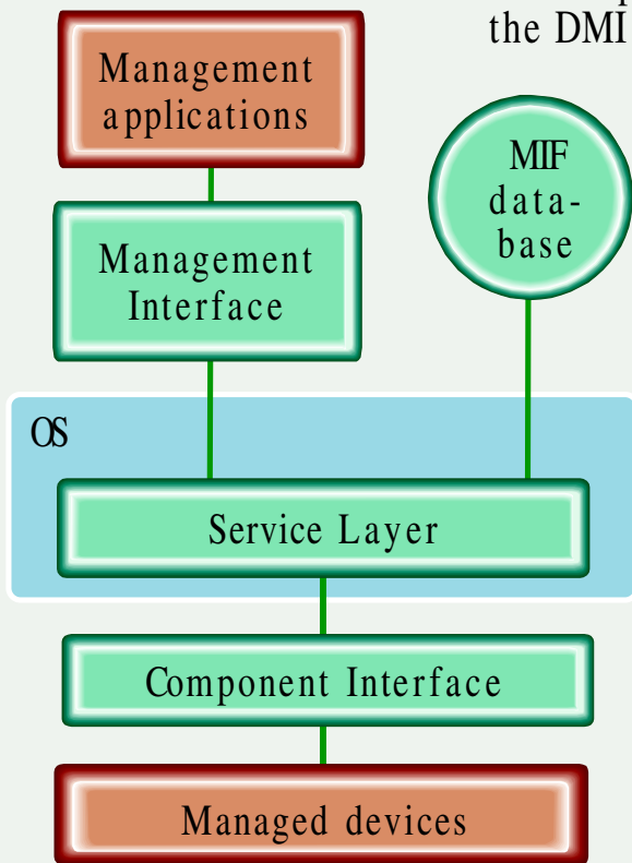
Windows 3.1 DMI implementation
