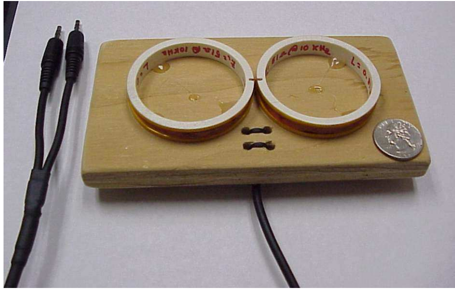
Figure 2: Inductive coil pair, optimized for 10\text{ kHz} and 2\text{ cm} depth.
